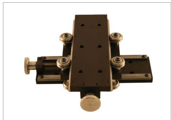
HCS-40-4X4 Dual Axis Slide Weight Capacity: 40 lb (18 kg) Slide Stroke: 4"x4" (100x100 mm)
