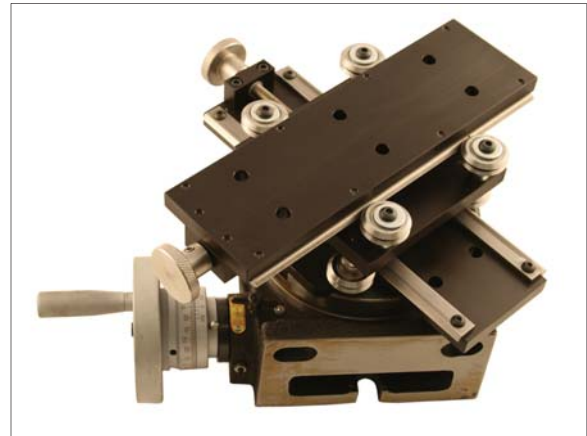
HCS-40-4X4-RT Hand Crank Rotary Table Weight Capacity: 40 lb (18 kg) Slide Stroke: 4"x4" (100x100 mm) Rotation: 360 degrees
