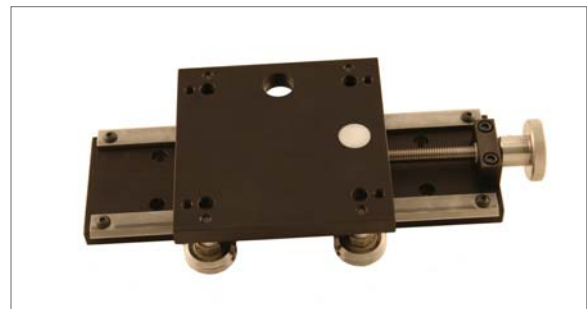
HCS-40-4 Single Axis Slide Weight Capacity: 40 lb (18 kg) Slide Stroke: 4" (100 mm)
